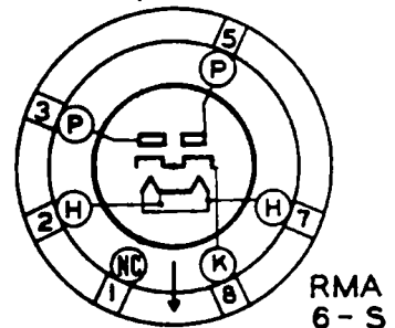
TUBE AND BASE DIAGRAM (BOTTOM VIEW)
